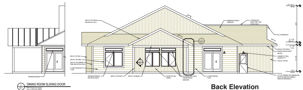
Back Elevation
